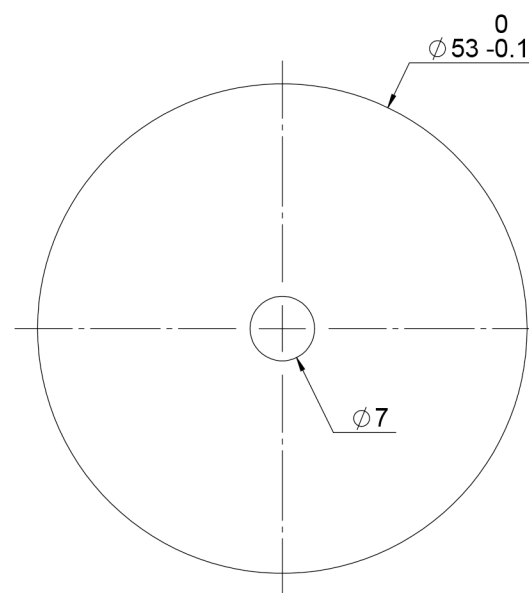
1G02817A IS6-WIDE ANGLE PORT Ø 7 APERTURE
