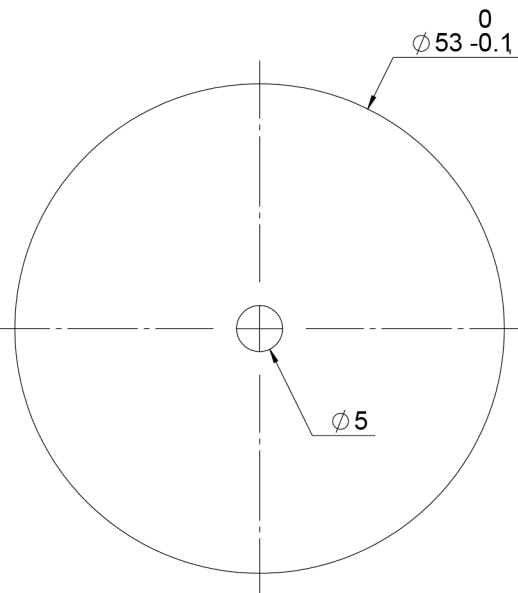
1G02802A IS6-WIDE ANGLE PORT Ø 5 APERTURE
