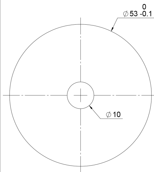
1G02801A IS6-WIDE ANGLE PORT Ø 10 APERTURE
